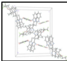
Fig. 2. Packing diagram of the title compound, [\text{C}_{16}\text{H}_{15}\text{F}_3\text{N}_3\text{OS}^+]_2 [\text{C}_6\text{Cl}_2\text{O}_4^{2-}] , viewed down the a axis. Dashed lines indicate strong \text{N-H}\cdots\text{O} and weak \text{C-H}\cdots\text{O} , \text{C-H}\cdots\text{F} intermolecular hydrogen bonds linking the [\text{C}_{16}\text{H}_{15}\text{F}_3\text{N}_3\text{OS}^+]_2 and [\text{C}_6\text{Cl}_2\text{O}_4^{2-}] ions into an infinite \text{O-H}\cdots\text{O-H}\cdots\text{O-H} chain network along the b axis in the (011) plane.
