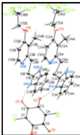
Fig. 1. Molecular structure of [\text{C}_{16}\text{H}_{15}\text{F}_3\text{N}_3\text{OS}^+]_2 [\text{C}_6\text{Cl}_2\text{O}_4^{2-}] , showing the atom labeling scheme and 50% probability displacement ellipsoids. Dashed lines indicate strong \text{N-H}\cdots\text{O} intermolecular interactions within the asymmetric unit. H atoms are presented as small circles of arbitrary radius.
